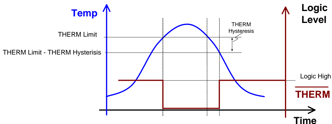
Figure 4.4 ADDR/ \overline{\text{THERM}} Output Response to Temperature Limit Exceeded
